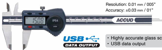
150 mm Dual Scale Splash Proof IP54 Digital Caliper
