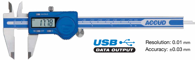
150 mm Dual Scale Digital Caliper
