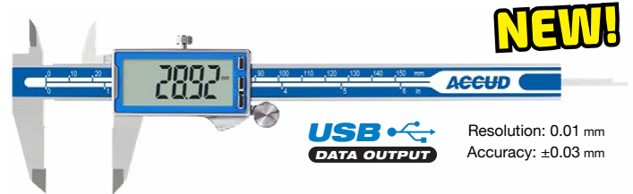
150 mm Dual Scale Digital Caliper
