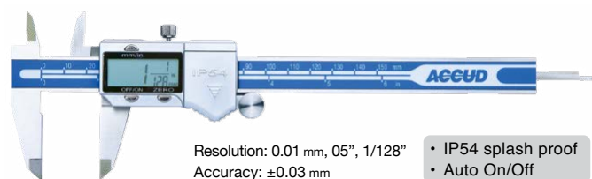
150 mm Fractional Imperial Digital Caliper
